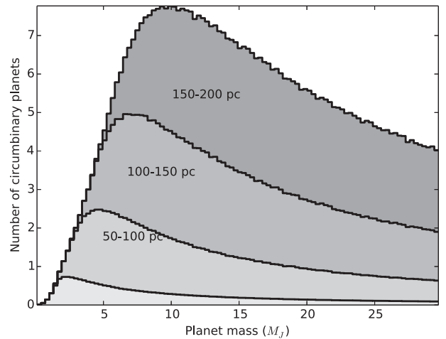
Figure 5. Mass histogram of detectable circumbinary planets. The four curves correspond to planets detected within spheres of \leq 50 pc (25 planets), \leq 100 pc (124 planets), \leq 150 pc (297 planets), and \leq 200 pc (516 planets).
