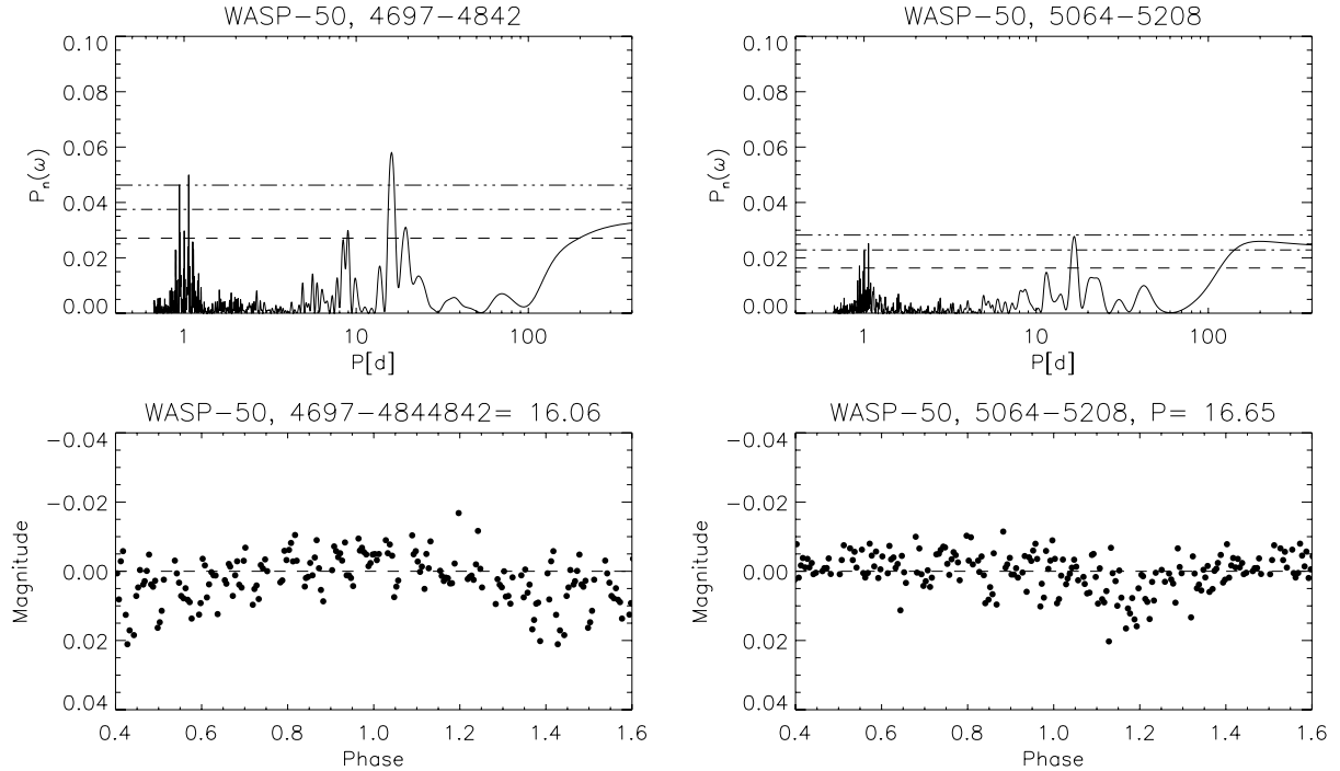
Fig. 2. Upper panels: periodograms for the WASP data from two seasons for WASP-50. The date range (JD–245 000) is given in the title of each panel. Horizontal lines indicate false alarm probability levels FAP = 0.1, 0.01, 0.001 . Lower panels: data folded and binned in 0.005 phase bins for the periods noted together with the date range in the plot title.
