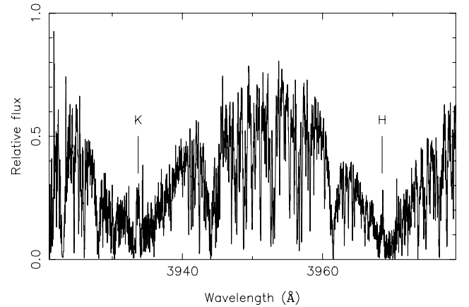
Fig. 6. A region of the co-added CORALIE spectrum of WASP-50 showing emission in the core of the CaII H and K lines.
