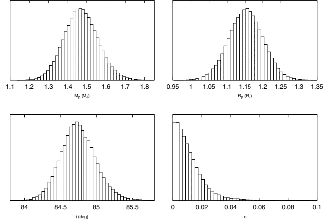
Fig. 7. Marginalized posterior distributions for the planet mass, radius, orbital inclination and eccentricity resulting from our global MCMC analysis.
