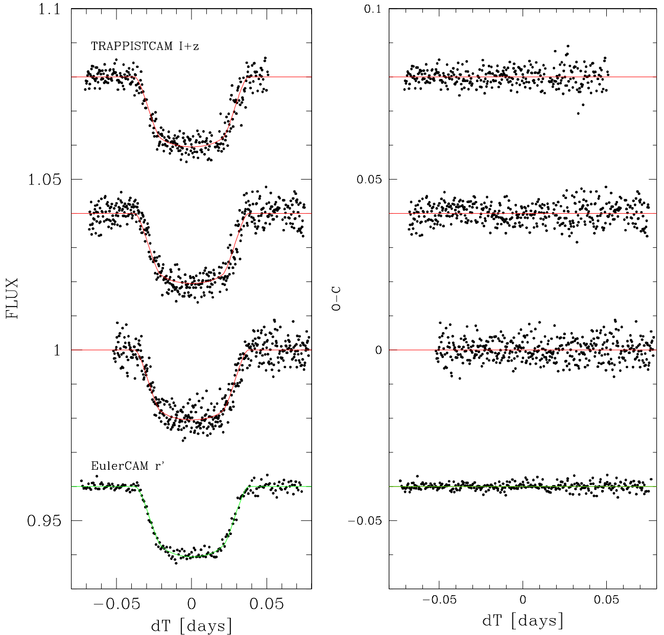
Fig. 3. Left, from top to bottom: period-folded TRAPPIST transit light curves of WASP-50 for 2010 December 23, 25, and 27, and Euler transit light curve. These light curves are divided by the best-fitting baseline models (see details in Sect. 4), and the best-fitting transit models are superimposed. Three light curves and models are shifted in the y -axis for the sake of clarity. Right: the residuals to the fit for each light curve.
