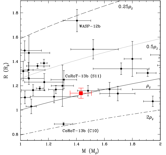
Fig. 8. Mass-radius diagram for the transiting planets with masses ranging from 1 to 2 M_{Jup} . WASP-50 b is shown as a square symbol. Two sets of values are shown for the planet CoRoT-13 b, the ones presented in the discovery paper (Cabrera et al. 2010, C10) and the ones recently reported by Southworth (2011, S11).
