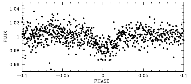
Fig. 1. WASP photometry of WASP-50 folded on the best-fitting transit ephemeris from the transit search algorithm presented in Collier Cameron et al. (2006), and binned per 5 measurements.
