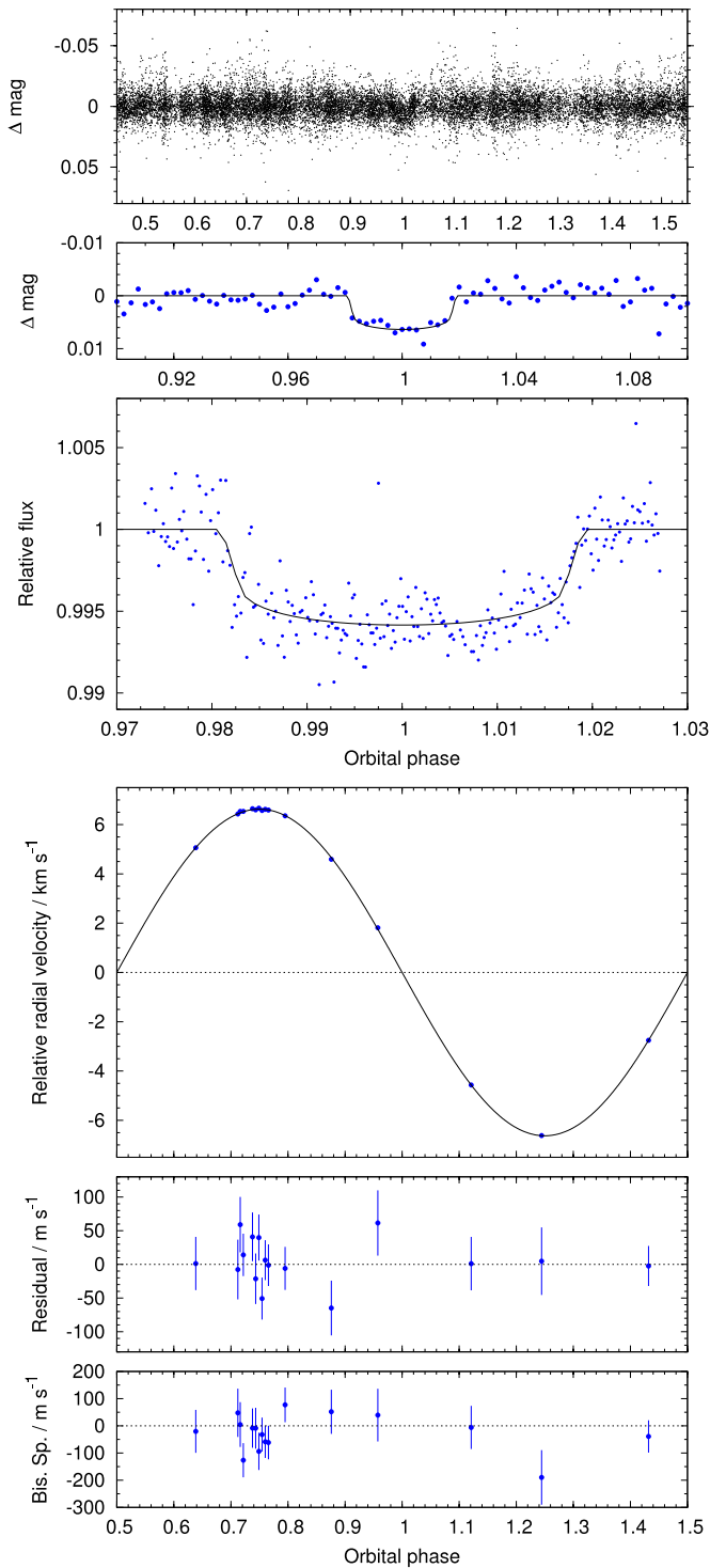
Figure 1. Top panel: WASP discovery light curve, folded on the ephemeris of Table 3. Second panel: binned ( \Delta\phi = 0.0025 ) WASP data around the transit. Third panel: transit light curve obtained with Euler. Fourth panel: relative RV measurements of WASP-30 measured by CORALIE. Fifth panel: residuals about the model RV solution. Bottom panel: bisector spans.
