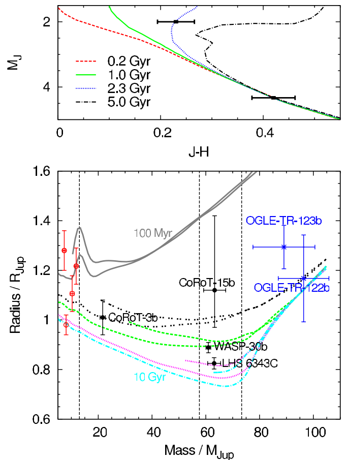
Figure 2. Top panel: color-magnitude diagram for WASP-30 and a nearby star with which it appears to be comoving. Isochrones for the ages shown are from Marigo et al. (2008). Bottom panel: mass-radius diagram showing objects in the mass range 5\text{--}110 M_{\text{Jup}} with precise radius measurements. The data are from http://www.inscience.ch/transits/ and, in the case of LHS 6343 C, from J. A. Johnson (2010, private communication). The theoretical isochrones with ages 0.1, 0.5, 1, 5, and 10 Gyr are from the DUSTY00 and COND03 models. Those that reach down to the minimum plotted mass are the COND03 isochrones. The vertical dashed lines depict the approximate theoretical minimum masses for deuterium burning ( 13 M_{\text{Jup}} ), lithium burning ( 0.055 M_\odot ), and hydrogen burning ( 0.07 M_\odot ; e.g., Chabrier et al. 2000a, 2000b).
